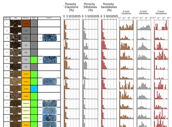
Example of PLANE[TechLab] technology application to cuttings (PLANE[CUTTING]). Synthetic logs with Geological (left) and windowed Digital Rock Physics properties (center and right), per lithology and properties distributions.
